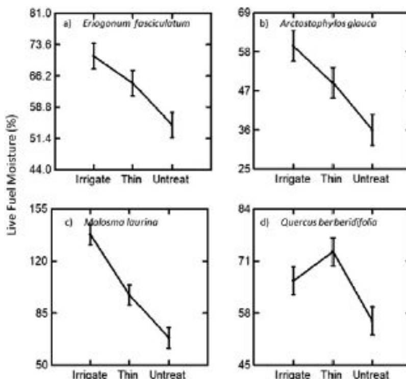
Fig. 5. Average LFM for all collections from June - October 2017 for the four species. Error bars are the standard error of the mean and ANOVA gave a significant difference between treatments for all species, though the Bonferroni test showed: a) Eriogonum fasciculatum : P < 0.001 , Irrigated = Thinned > Untreated, b) Arctostaphylos glauca : P = 0.004 , Irrigated > Thinned > Untreated, c) Malosma laurina : P < 0.001 , Irrigated > Thinned > Untreated, and d) Quercus berberidifolia : P = 0.04 , Irrigated = Thinned > Untreated.
