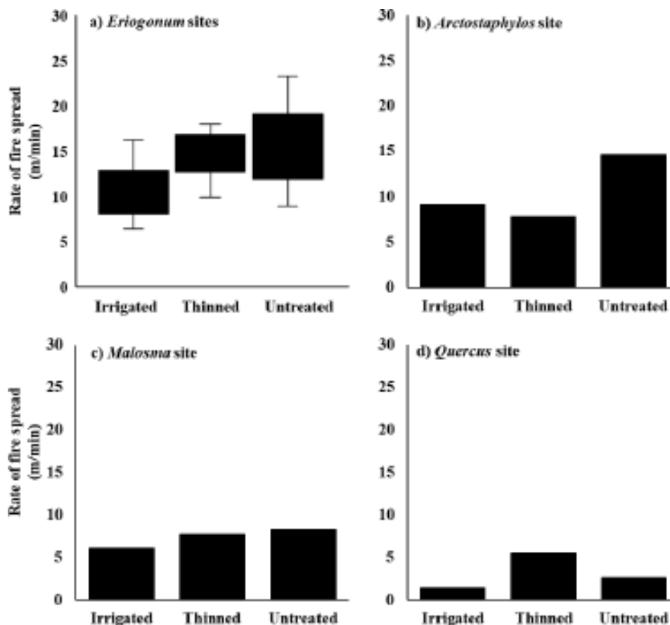
Fig. 7. Predicted rate of fire spread for the dry season for a) Eriogonum , error bars are the standard error of the mean across the three sites, b) Arctostaphylos , c) Malosma , and d) Quercus sites for the three treatments.
